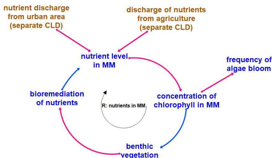
Figure 3 Top-level "Nutrients in Mar Menor" CLD
